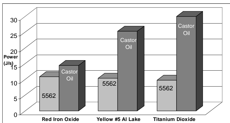
Figure 1. Silicone carbinol fluid requires less equipment power than castor oil to suspend pigments..
