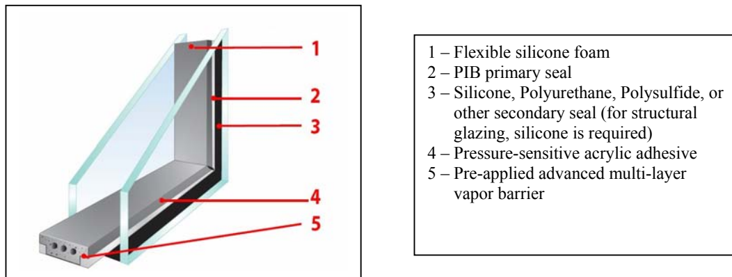
Figure 9 – Novel silicone foam warm-edge spacer design with integrated polyisobutylene primary seal (Courtesy of Edgetech I.G. Inc., Cambridge, Ohio, U.S.A., www.edgetechig.com/ )
