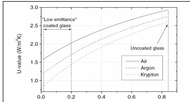
Figure 1 – U-value calculated according to EN 673 9 versus emittance for the third surface (counted from the outside) and for different gas fill (12 mm spacer width). Low emittance glazings have emittance values below 20% (0.2) and uncoated glass has about 84% (0.84) 10
