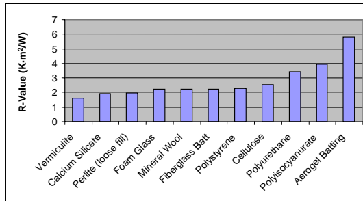
Figure 5 – Thermal resistance (R-value in \text{K}\cdot\text{m}^2/\text{W} ) for different insulation materials
