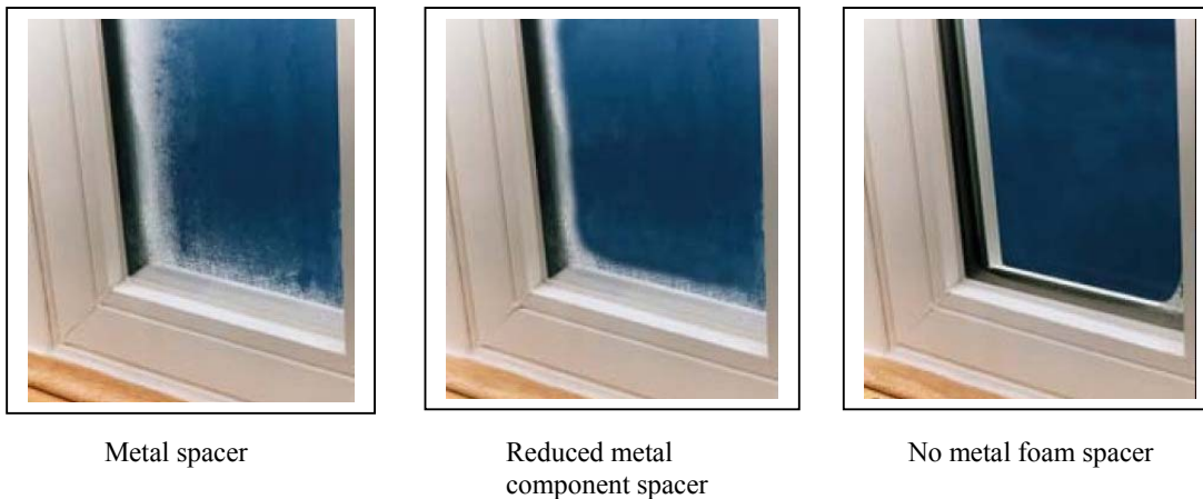
Figure 2 – Condensation and frost forming on interior pane for different spacer systems (Courtesy of Edgetech I.G. Inc., Cambridge, Ohio, U.S.A., www.edgetechig.com/ )
