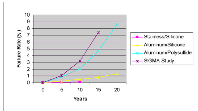
Figure 11 – Cumulative field failure rates after up to 20 years of field service (adapted from 54 )
