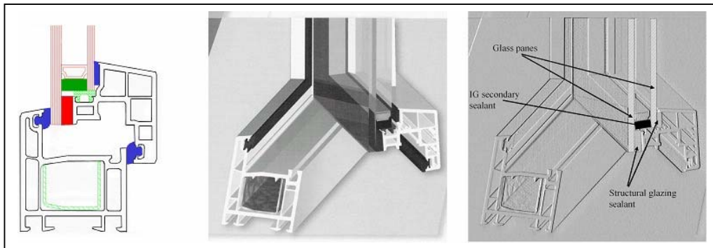
Figure 12 – Structurally bonded uPVC window system (Courtesy of Profine International, Profine GmbH International Profile Group, Troisdorf, Germany, website: http://www.profine-group.de/ )
