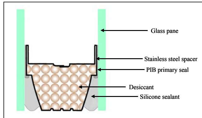
Figure 10 – Proprietary PIB/silicone dual-seal design based on patented stainless steel spacer (adapted from 30 )
