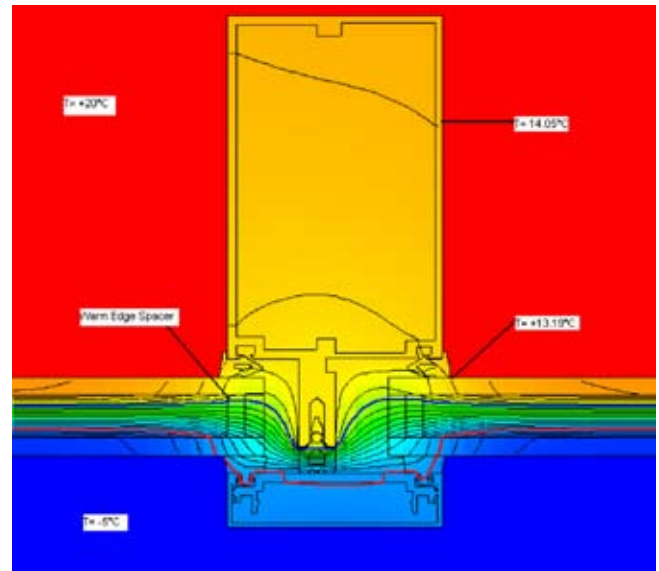
Figure 3.2 Mechanically fixed with warm edge IG, aged installation
