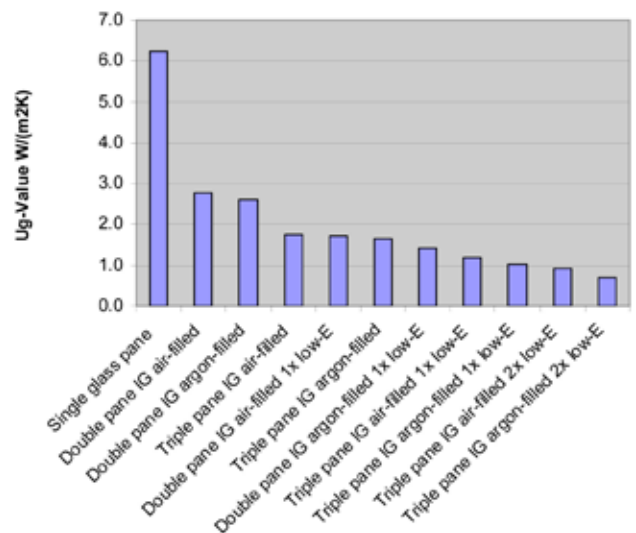
Figure 1 U value of various types of glazing assemblies
