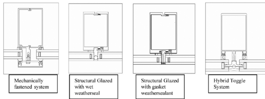
Figure 2 Types of frame and fastening systems.
