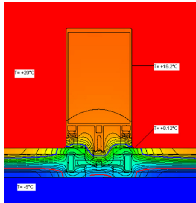
Figures 3.1-3.5 Thermal inclines of each design with a warm edge spacer.
