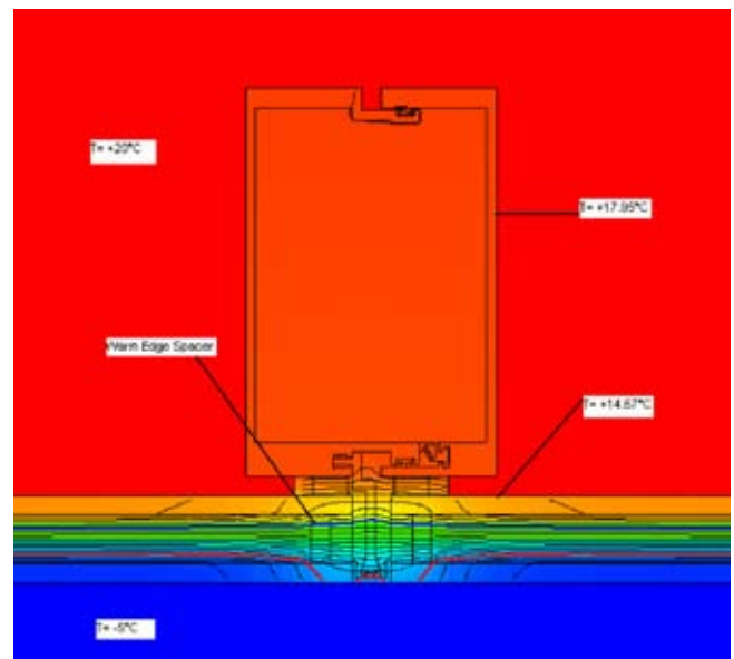
Figure 3.4 Structurally glazed with warm edge IG and dry gasket weatherseal
