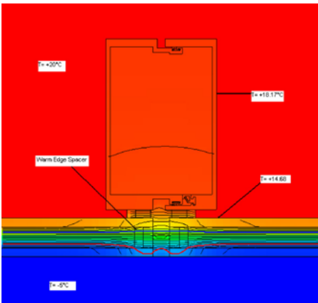
Figure 3.3 Structurally glazed with warm edge IG and wet weatherseal
