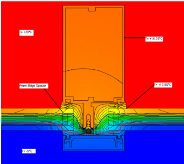
Figure 3.1 Mechanically fixed with warm edge IG, new installation
